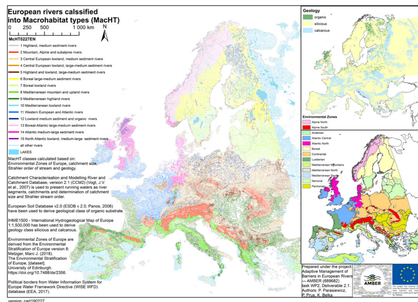
Figure 4. European rivers classified into 15 Fish Community Macrohabitat types (FCMacHT) (AMBER D2.1, version 2.0).
