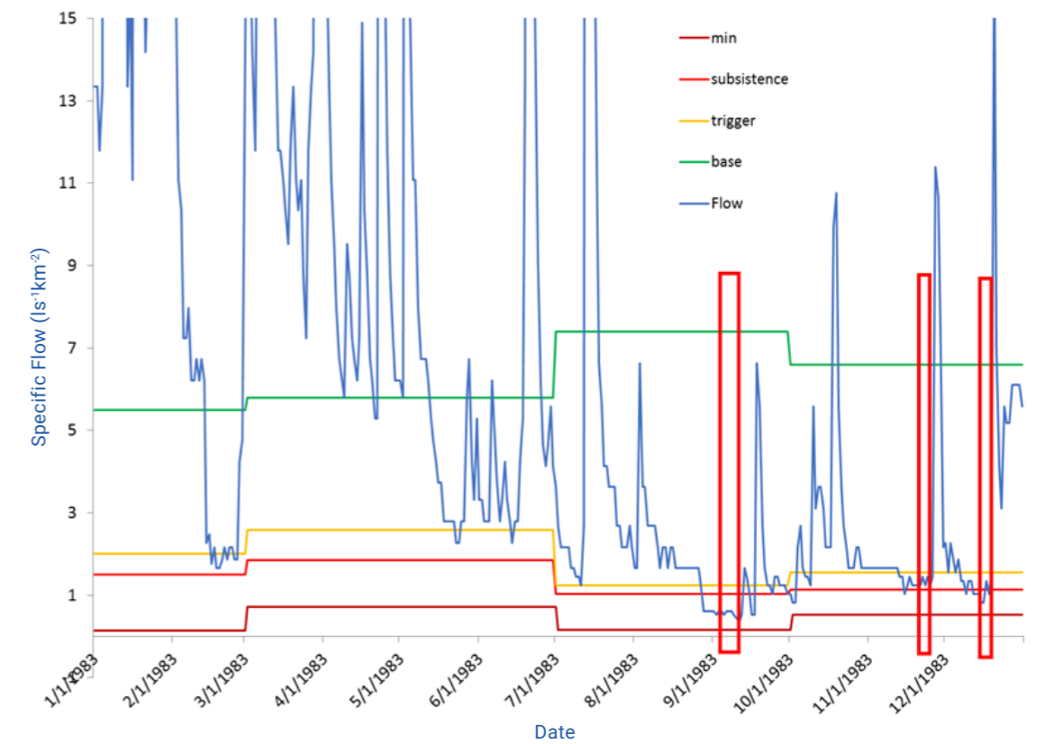
Figure 26. Example of application of dynamic augmentation rules in E-Flows management.
