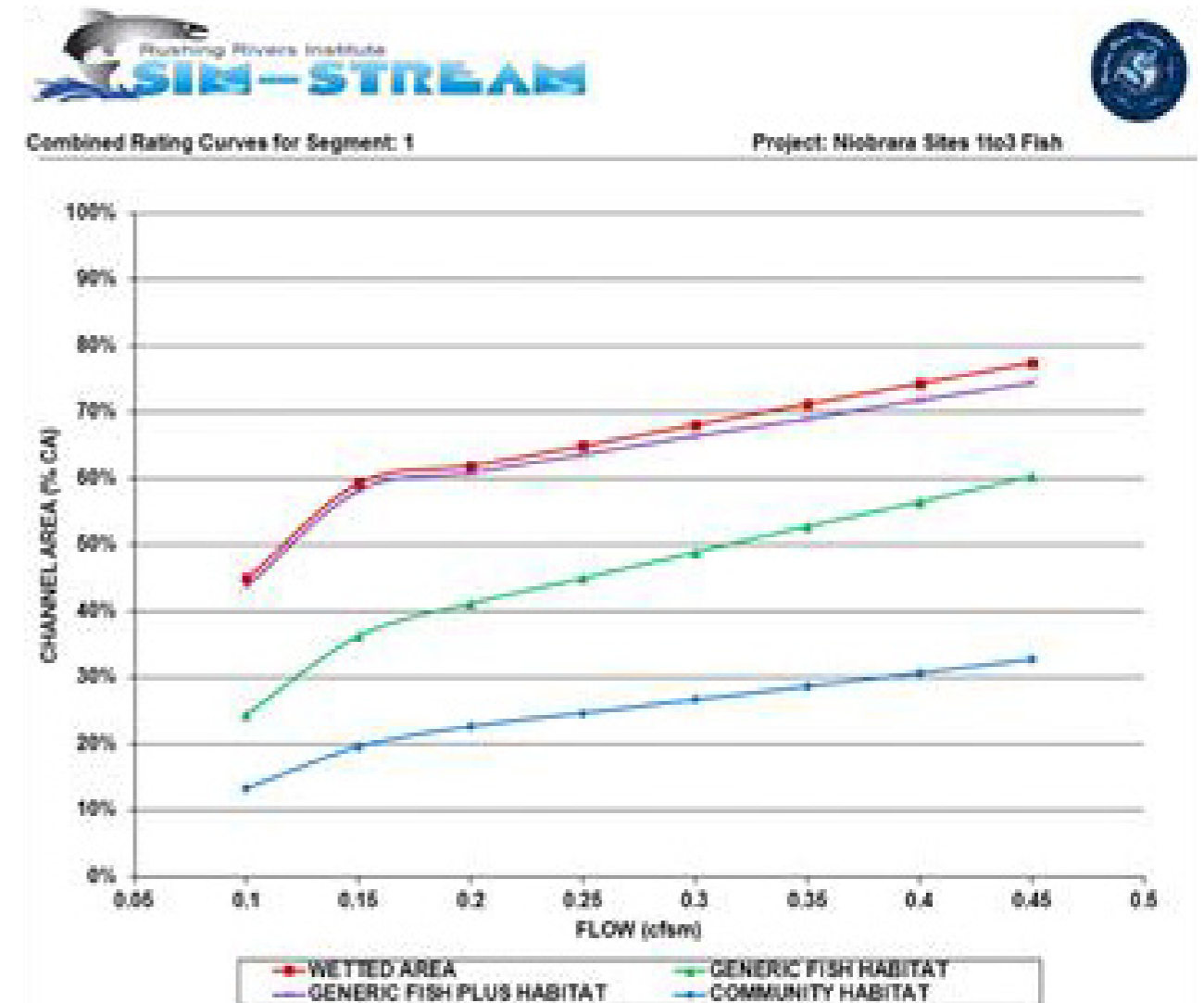
Figure 30. Community rating curves for Segment 1 (Sites 1-3) in the Niobrara River.
